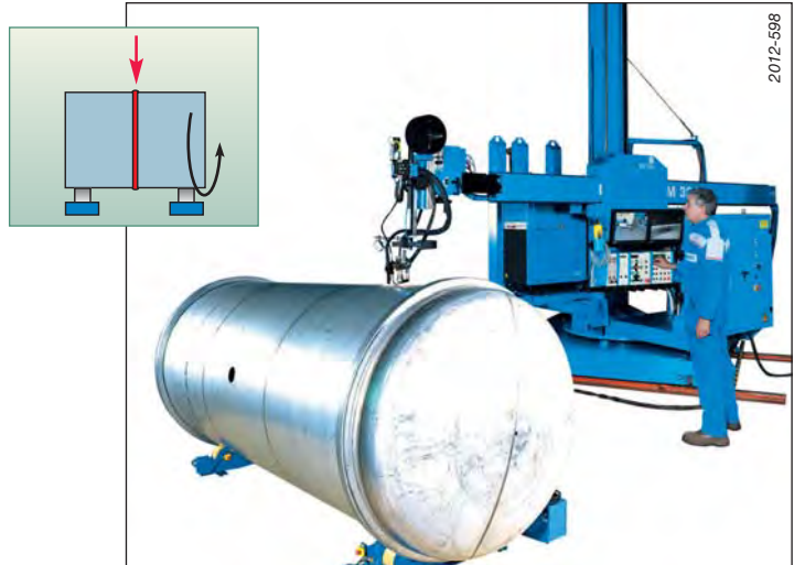
Circular welding with column and boom on rotator or positioner.
